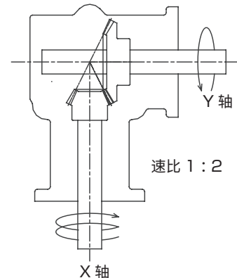
Bevel Gearboxes
